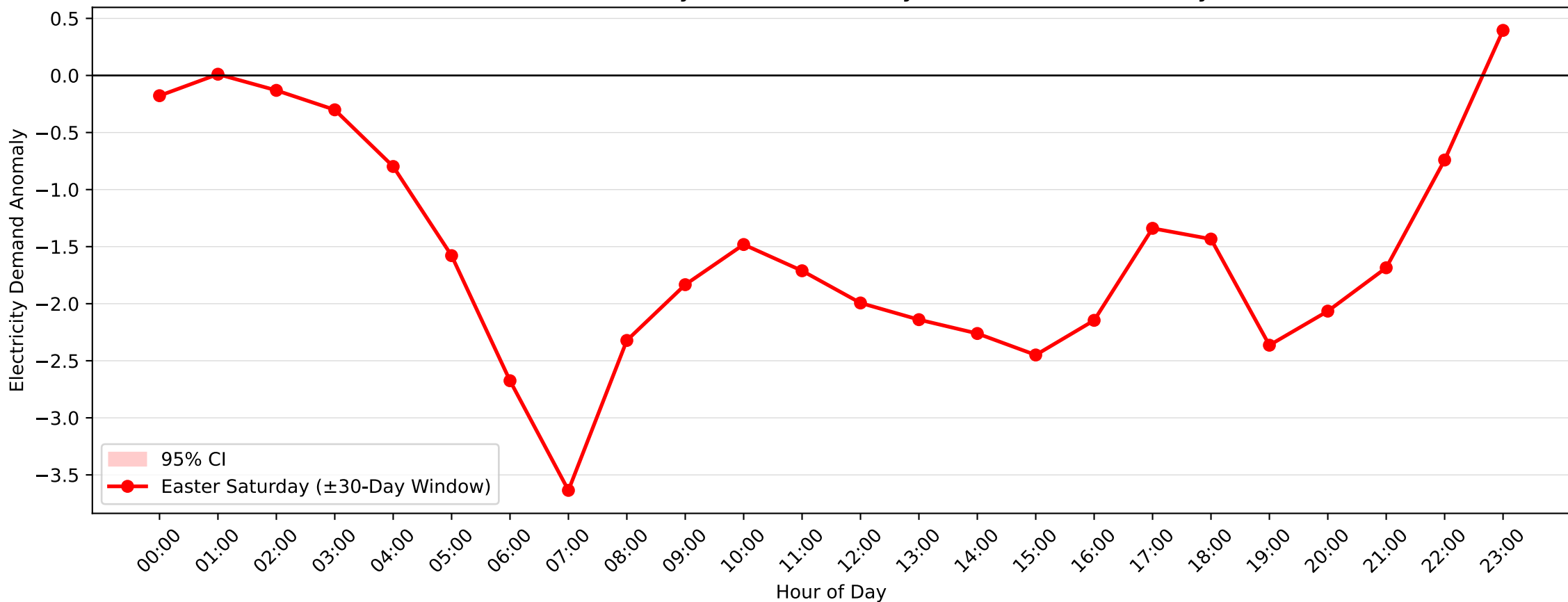
Five Dock Demand Anomaly: Easter Saturday (2010-2011, \pm 30 -Day Window)
