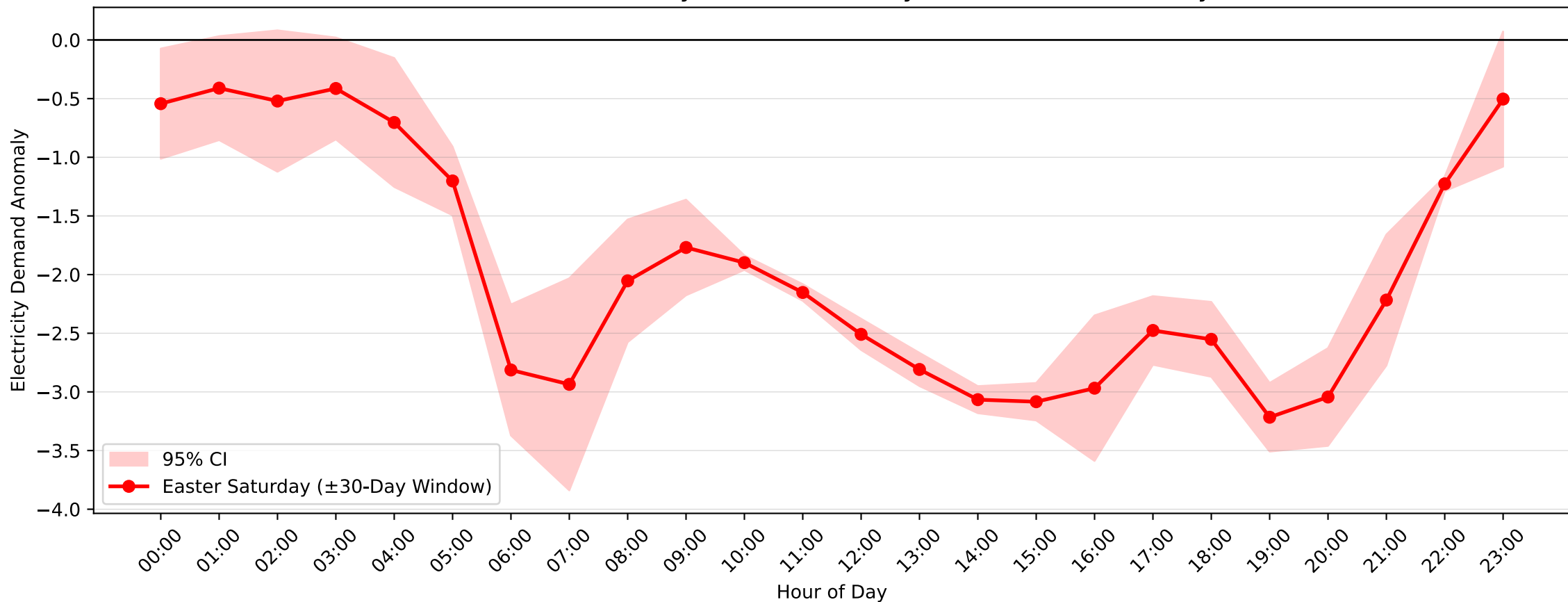
Five Dock Demand Anomaly: Easter Saturday (2006–2007, \pm 30 -Day Window)
